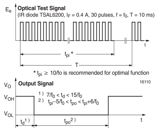
Figure 1. Output Function
